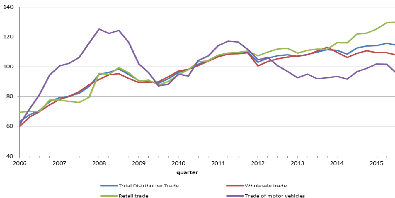
Indices of Distributive Trade Turnover, seasonally adjusted series BiH (2010=100)
