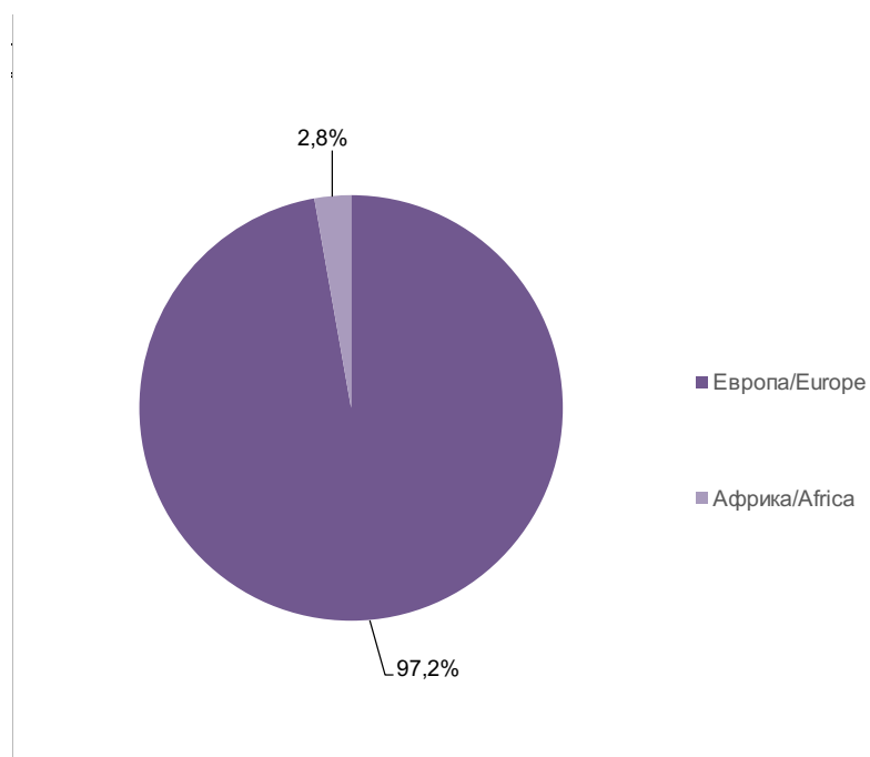
Figure 1 VALUE OF PERFORMED CONSTRUCTION WORKS, FOURTH QUARTER 2023, % SHARE
