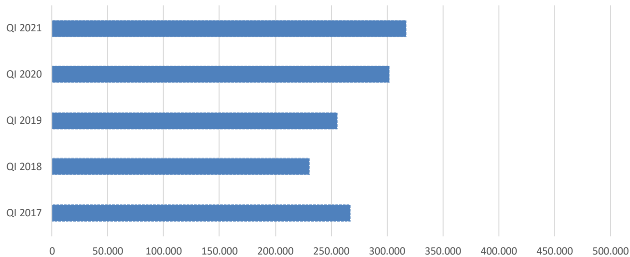
Graph.2.4. MMS sent
